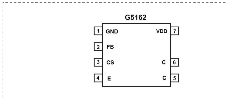
Pin Configuration: G5162 Series ( SOIC-7 )
