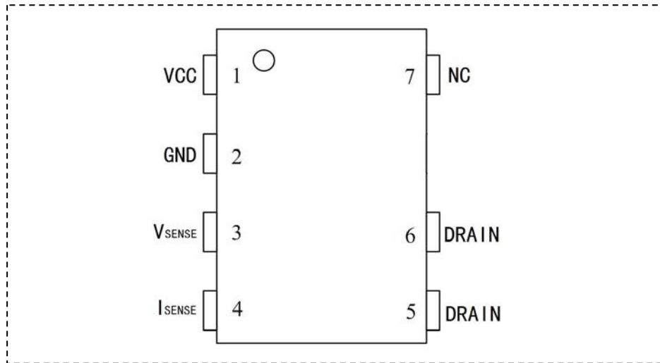
Figure2.1: G5236F Series (SOP7 Package)
